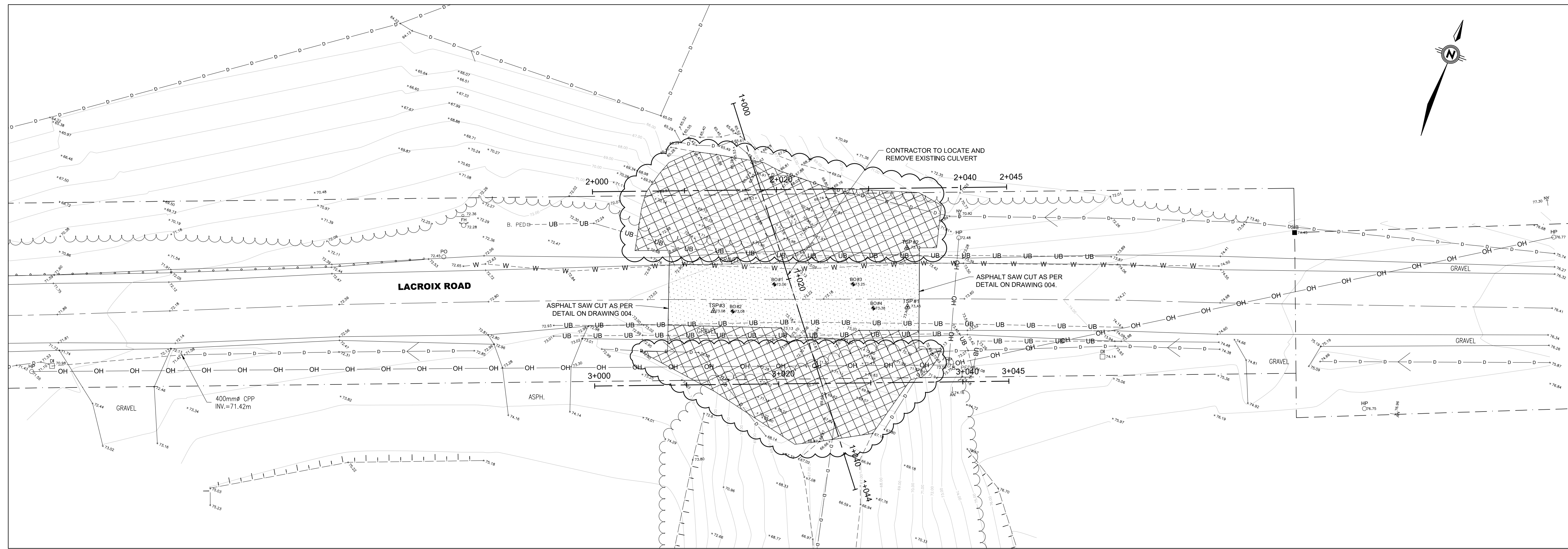
REMOVALS SCALE 1:250
