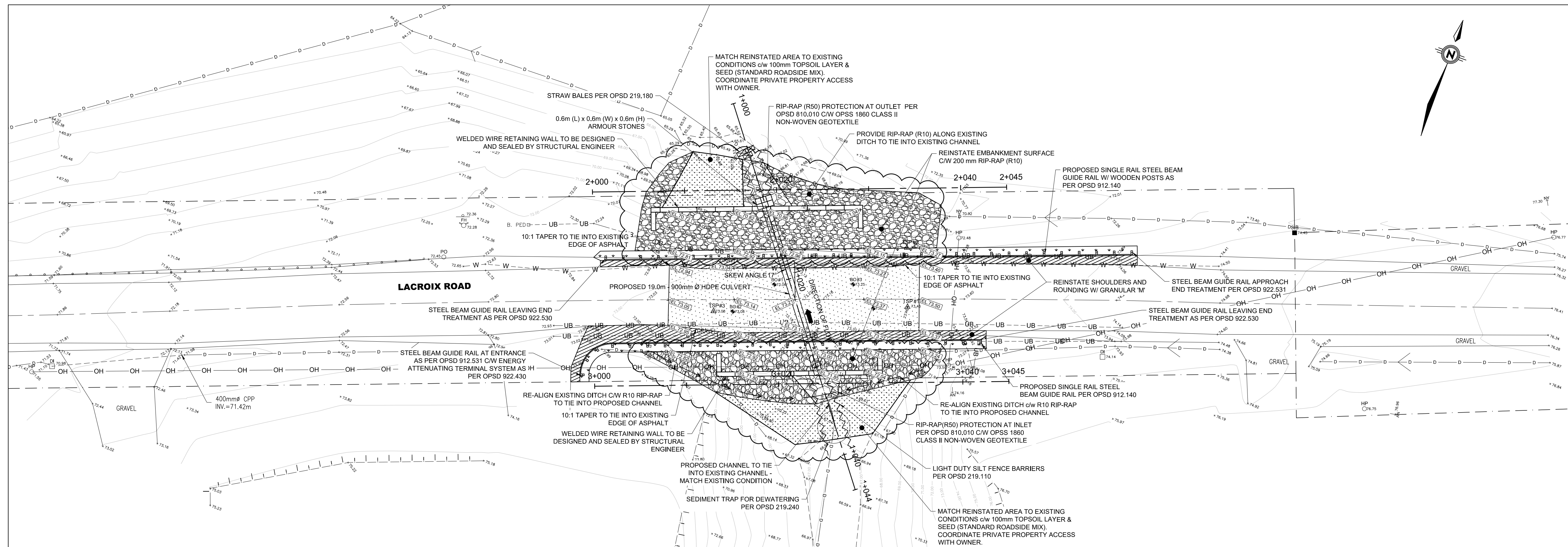
REINSTATEMENTS SCALE 1:250
